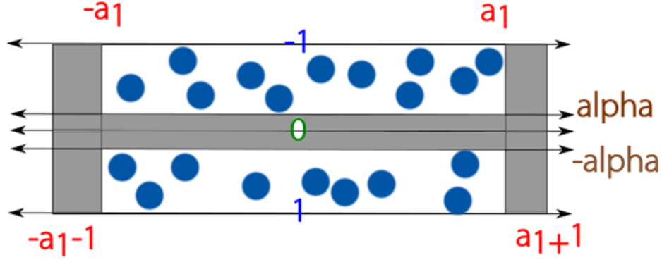
Figure 7: Changing the weight moves the Mellin contour. The index is constant while the contour remains in a pole-free strip and jumps by the algebraic multiplicities of the enclosed indicial roots when a pole is crossed.
