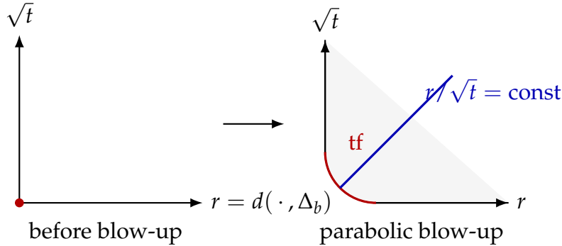
Figure 11: The temporal diagonal is parabolically blown up. The new face keeps the heat variable r/\sqrt{t} finite and carries the Gaussian model.
