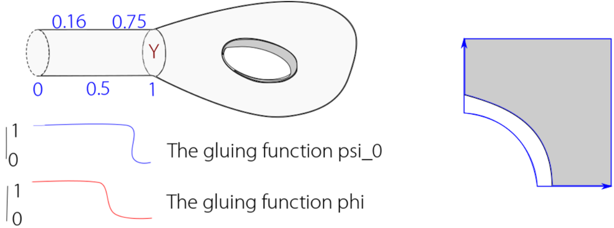
Figure 12: Left: compatible cutoffs separate the compact interior from the product cylinder while retaining an overlap on which the two model kernels can be compared. Right: after lifting to the b -double space, the boundary correction is supported near the front face and away from the opposite side face. This support control makes the alternating temporal and boundary corrections compatible.
